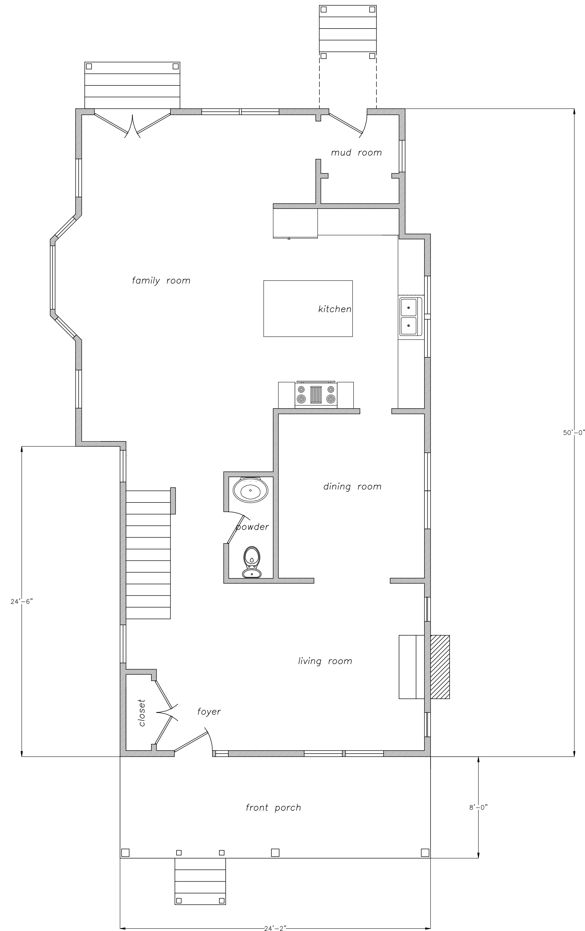
Proposed 1st Floor Plan Scale: 1/4" = 1'-0" actual floor area = 1,338 square feet City Area: 1320 square feet (not including bay)
